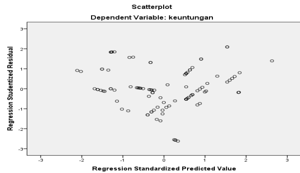
Figure 1. Test of Heteroscadasticity
